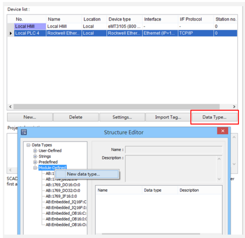
Fig.11 Structure Editor
